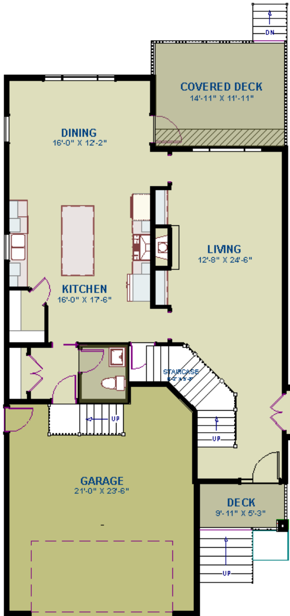
LIVING AREA 1163 SQ FT
